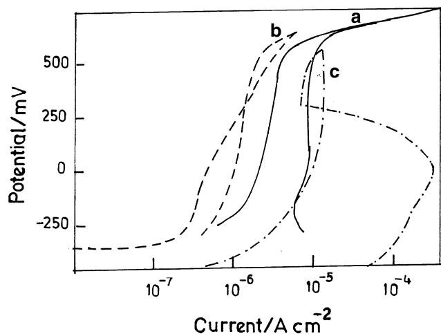
Fig. 2 Cyclic polarisation curves for steel in cement extracts. (a) OPC (900 ppm Cl - ), (b) PPC (900 ppm Cl - ) and (c) PSC (2000 ppm Cl - )
